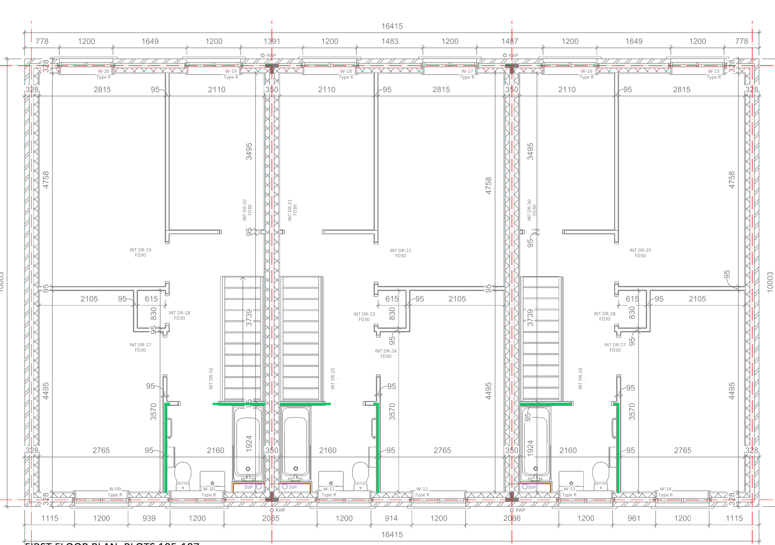
FIRST FLOOR PLAN: PLOTS 105-107
