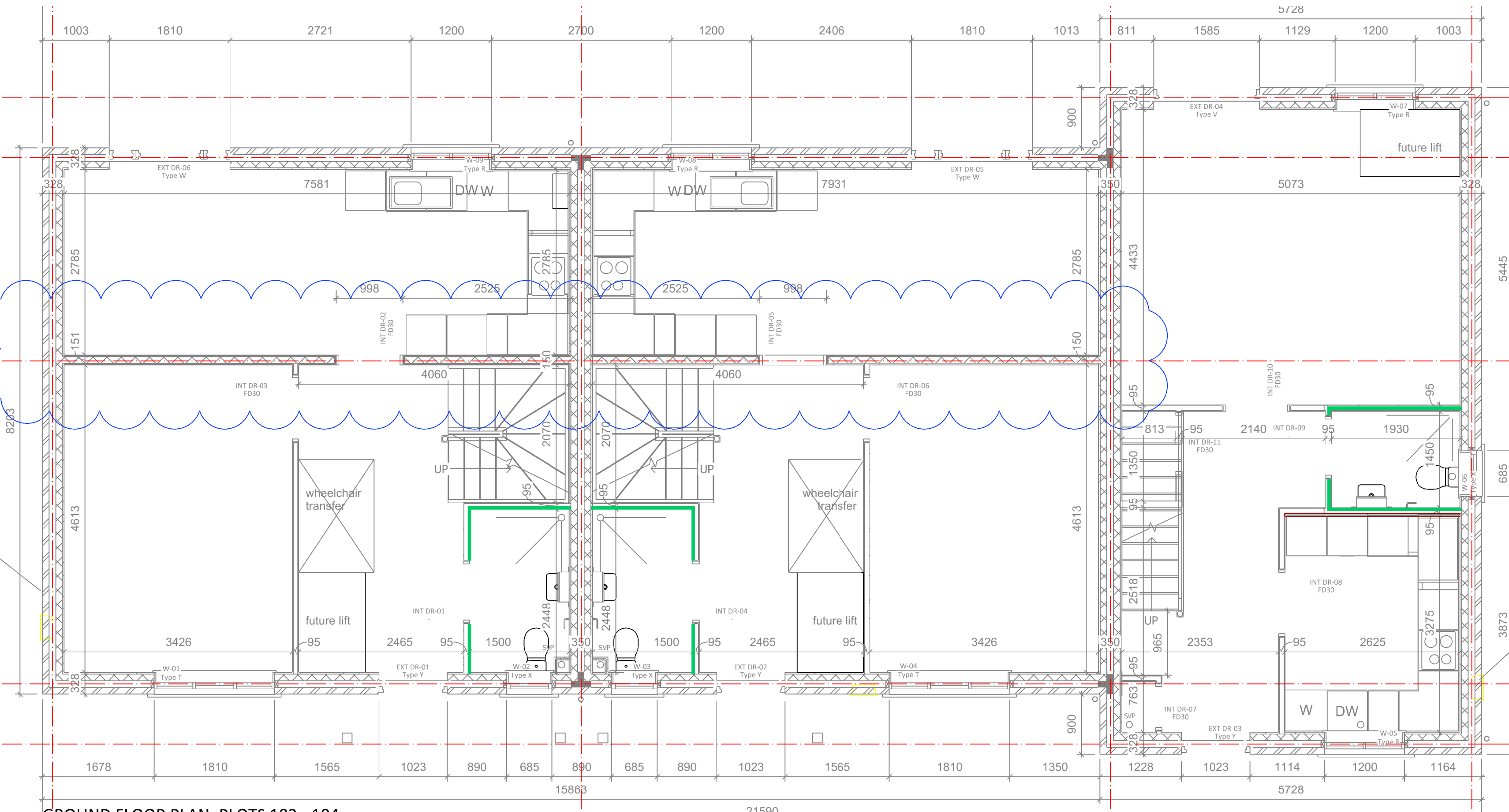
GROUND FLOOR PLAN: PLOTS 102 - 104
