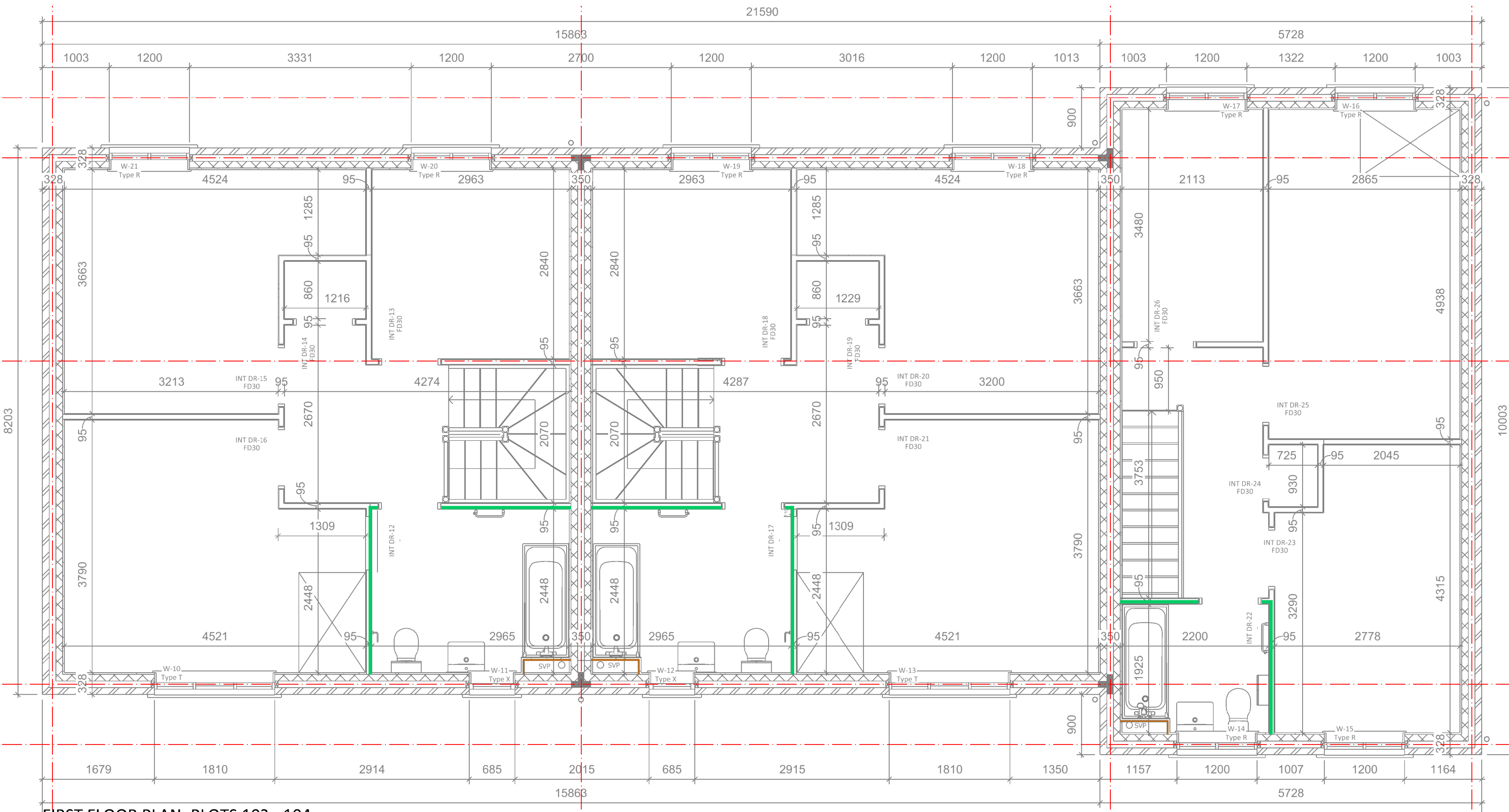
FIRST FLOOR PLAN: PLOTS 102 - 104
