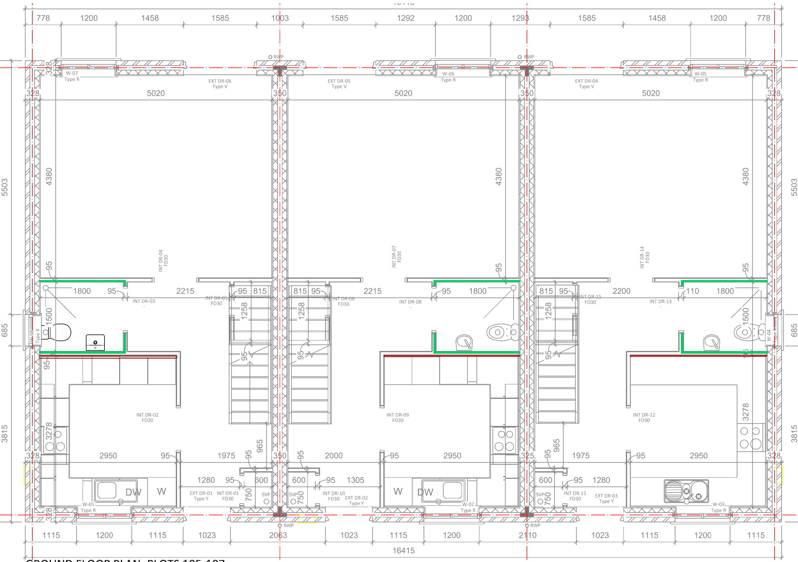
GROUND FLOOR PLAN: PLOTS 105-107
